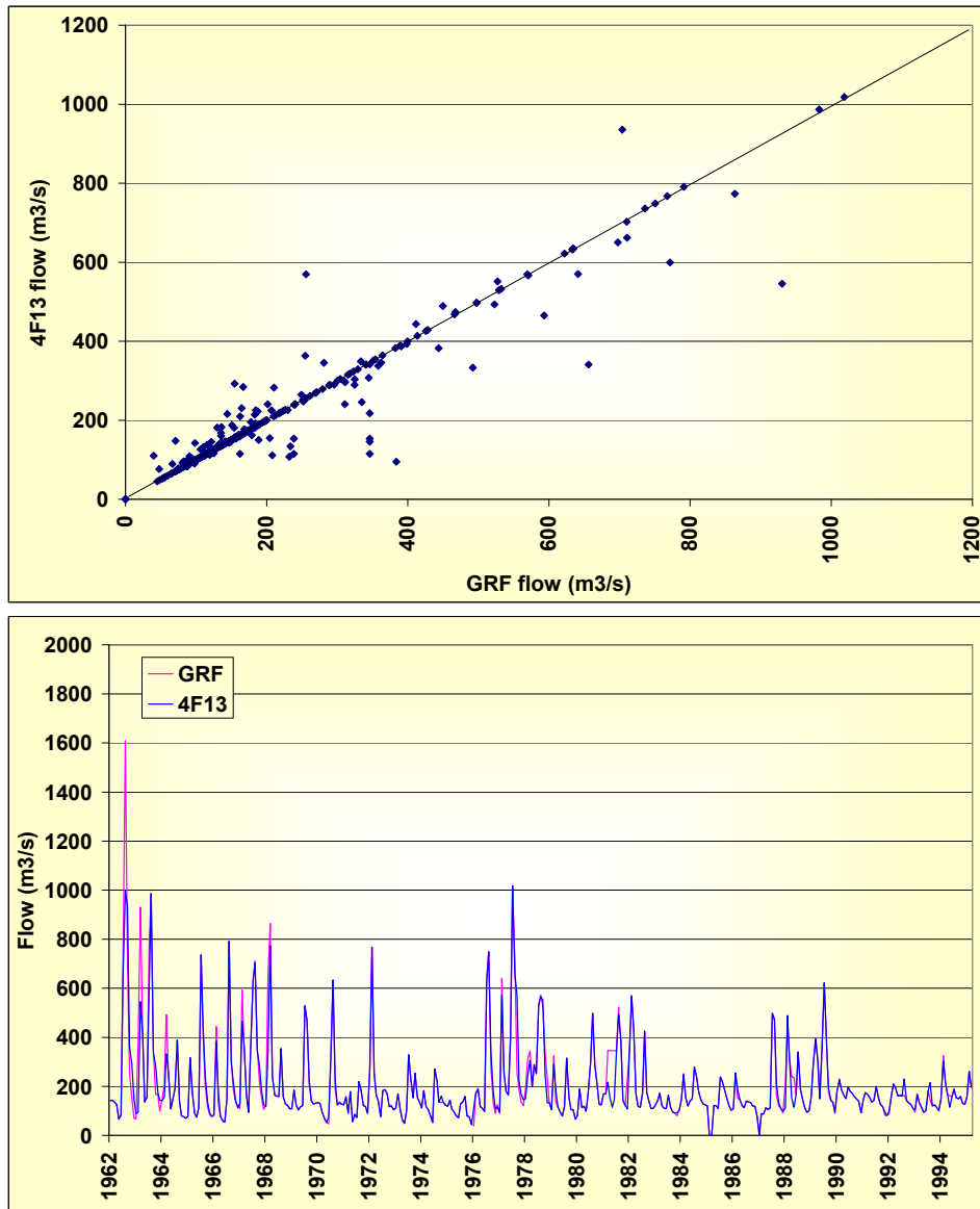
Figure 33. Comparison between similar data from two sources at Grand Falls. GRF originates from Global Runoff Discharge Data and 4F13 from University of Nairobi.
