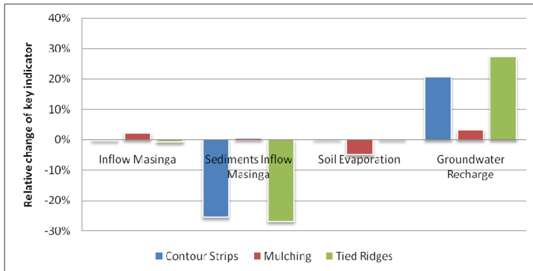
Figure 59: Relative changes of some of the key indicators for the 3 scenarios compared to the baseline situation (2005, dry)
