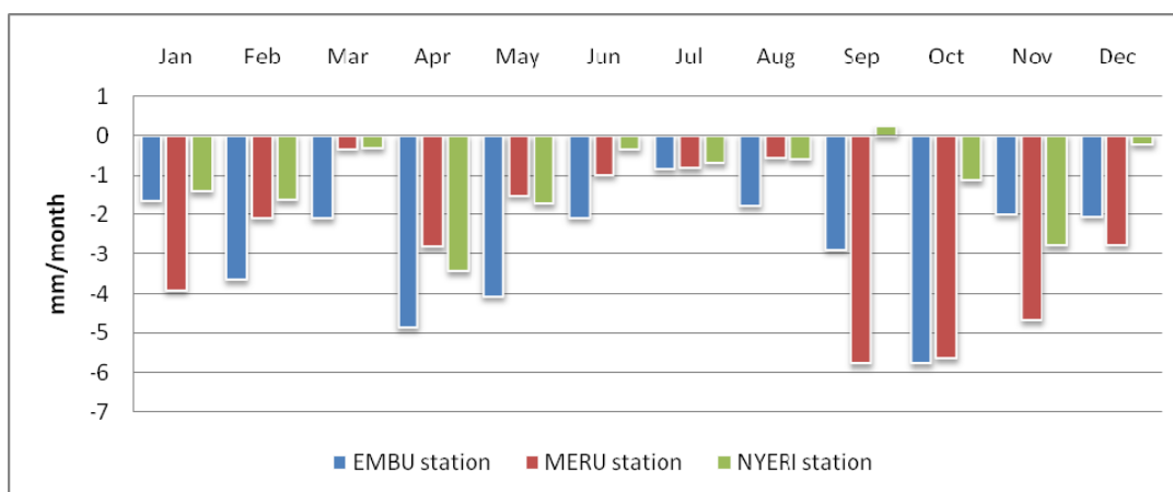
Figure 19: Residual (estimate - observed) mean per month of the 3 stations
