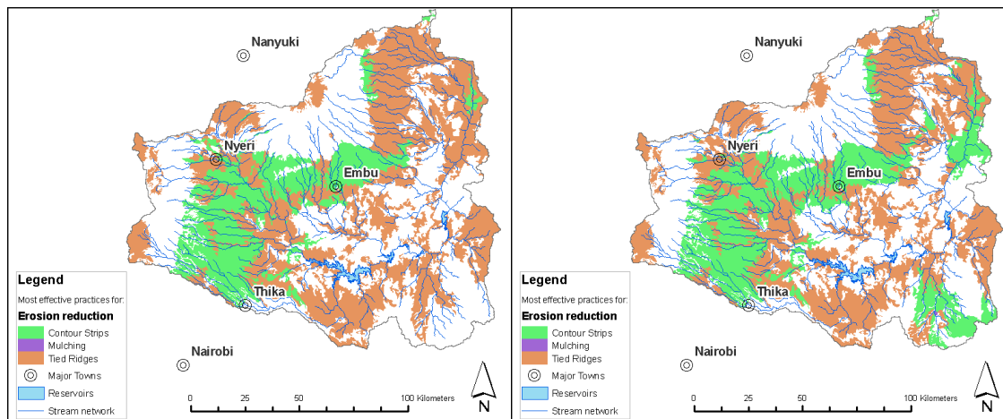
Figure 68: Spatial distribution of most effective practices reducing erosion for a dry year (left) and a wet year (right).
