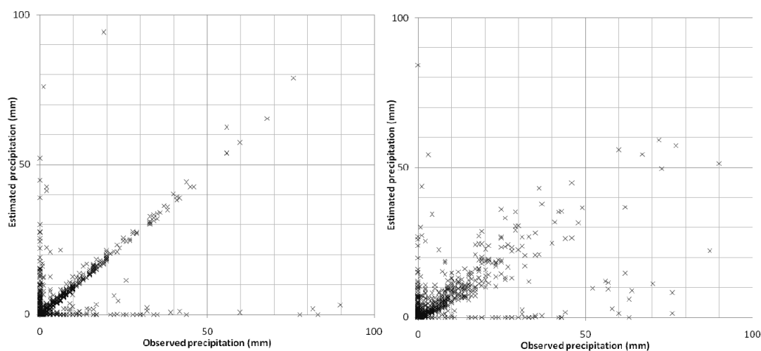
Figure 16: Scatterplots of observations (GSOD) and the estimates (FEWS) of the Nyeri station (left) and the Embu station (right)
