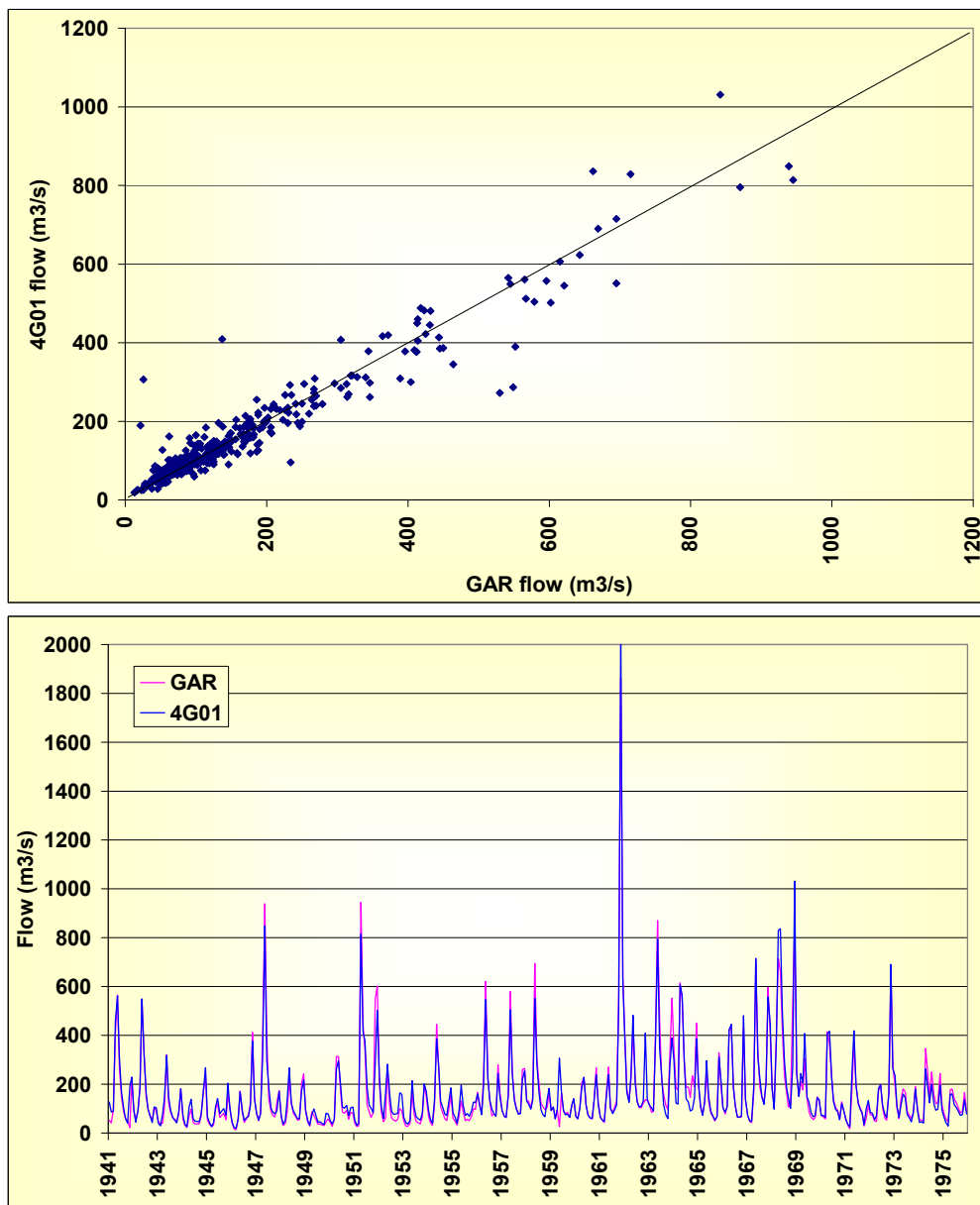
Figure 32. Comparison between similar data from two sources at Garissa. GAR originates from Global Runoff Discharge Data and 4G01 from University of Nairobi.
