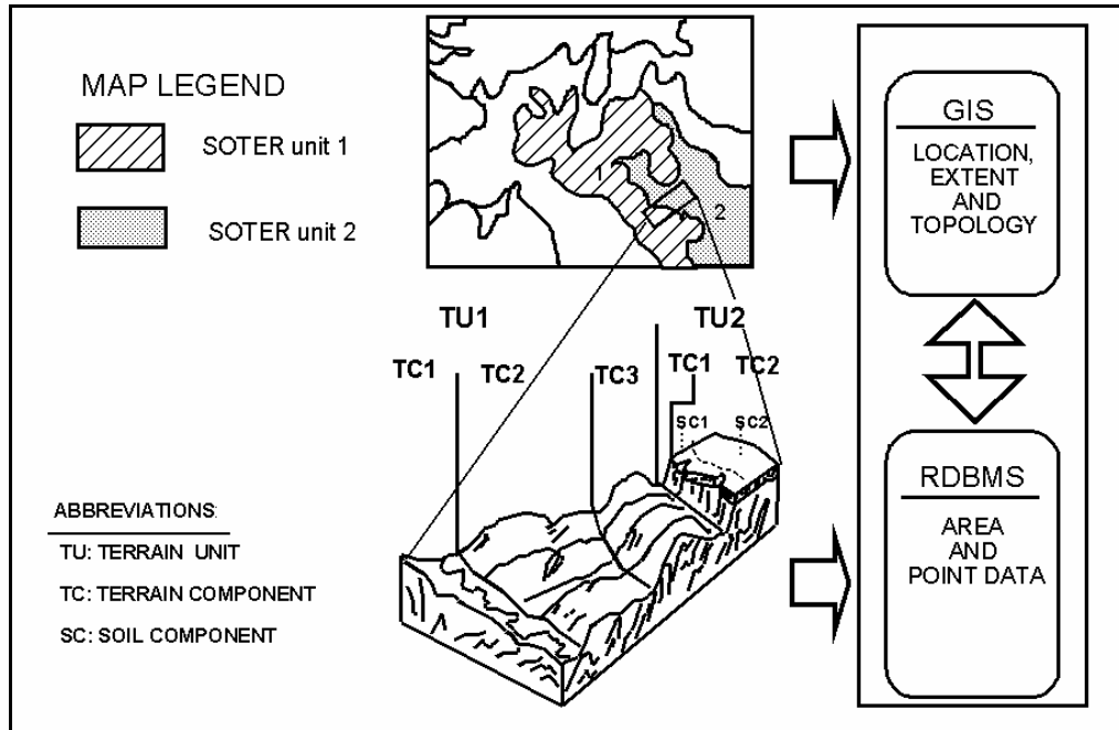
Figure 1. Schematic representation of two SOTER units and their terrain and soil components
