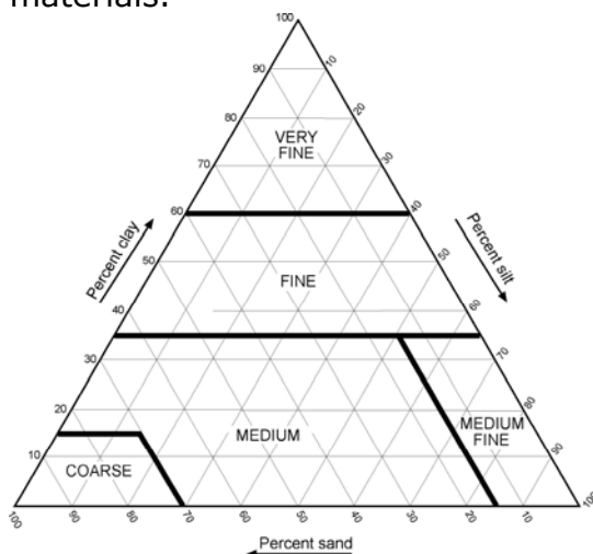
Figure 4. Soil texture classes
