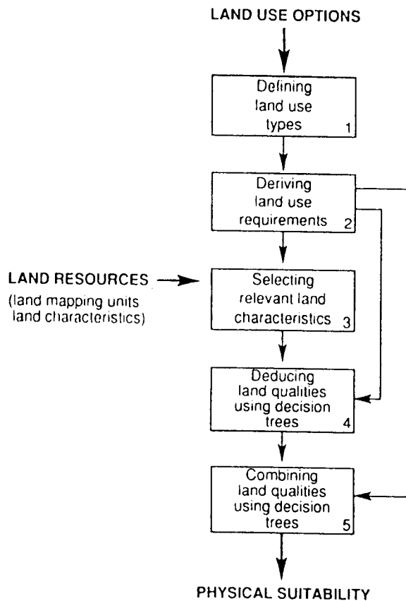
Figure 3: Relational diagram for assessing the physical suitability in ALES. (From van Lanen, 1991).
