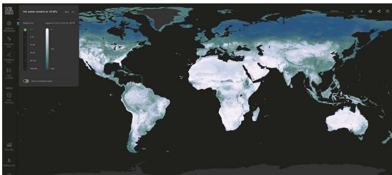
Volumetric water content at -33KPa from SoilGrids 2.0 (Turek et al, 2023).
